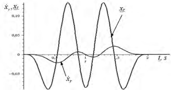
Figure 8 – Relative motion graphics using U_e(t) = a \sin^3(pt) ( n = 0 )
