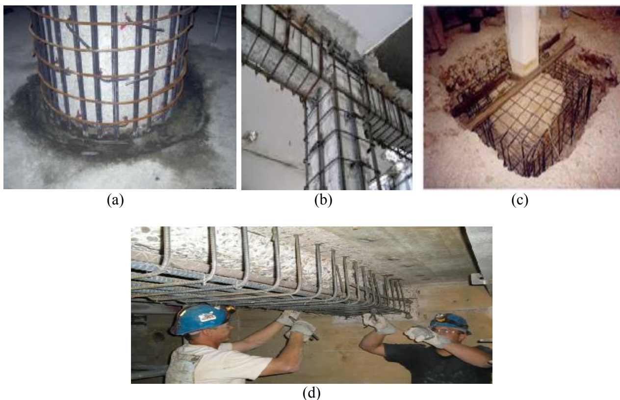
Figure 1 – RC jacketing of column (a), column and beam joint (b), footing (c) and beam (d)
